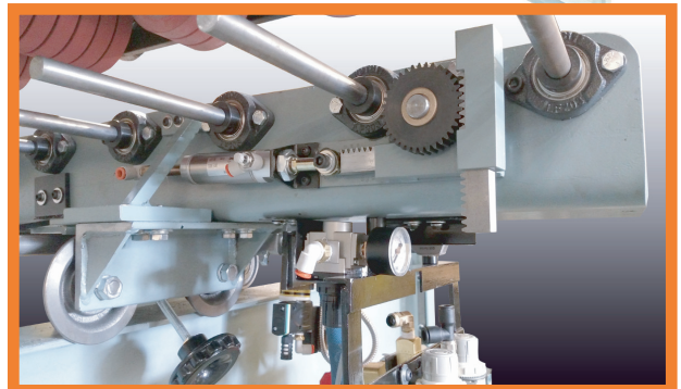
Alignment/Squaring mechanism
